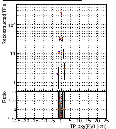
N of associated tracks (simToReco) vs dxy(PV)
