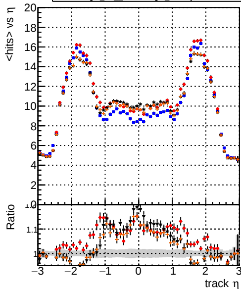
mean hits vs \eta Legend: DQM TT mkFit-DQM original (blue line), /data2/legianni/standalone-May24/CMSSW_13_2_X_X-2023-06-05-1100/src/DQM TT mkFit-DQM_mod_updatedmod-127 (red line), DQM TT mkFit-DQM_update-mod127 (black line), DQM TT mkFit-DQM_127-updatemod127 (orange line)
