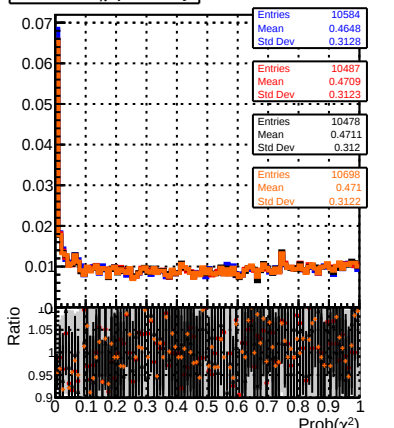
normalized \chi^2 probability
