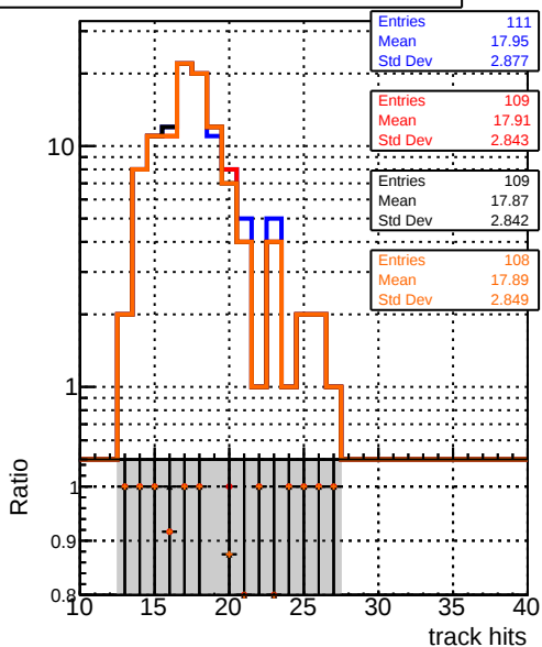
— DQM TT_mkFit-DQM original — /data2/legianni/standalone-May24/CMSSW_13_2_X_2023-06-05-1100/src/DQM TT_mkFit-DQM_mod_updatedmod127 — DQM TT_mkFit-DQM_update-mod127 — DQM TT_mkFit-DQM_127-updatemod127
