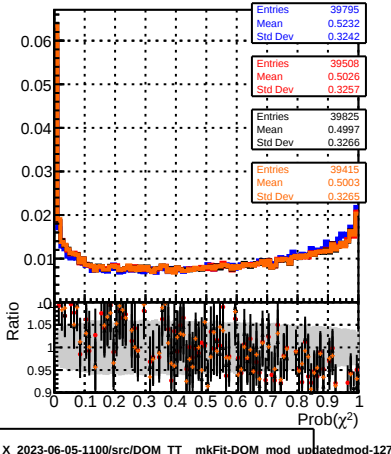
normalized \chi^2 probability
