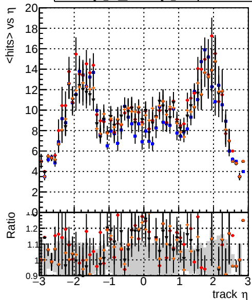
Legend: - DQM_TT_mkFit-DQM_original (blue line) - /data2/legianni/standalone-May24/CMSSW_13_2_X_2023-06-05-1100/src/DQM_TT_mkFit-DQM_mod_updatedmod127 (red line with dots) - DQM_TT_mkFit-DQM_update-mod127 (black line with dots) - DQM_TT_mkFit-DQM_127-updatemod127 (orange line with dots)
