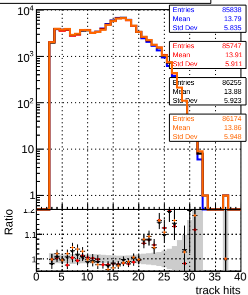
Legend: DQM TT mkFit-DQM original (blue line), /data2/legianni/standalone-May24/CMSSW_13_2_X_2023-06-05-1100/src/DQM TT mkFit-DQM_mod_updatedmod127 (red line), DQM TT mkFit-DQM_update-mod127 (black line), DQM TT mkFit-DQM_127-updatemod127 (orange line)
