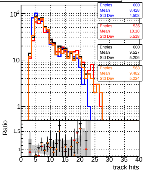
Legend: - DQM TT mkFit-DQM original (blue line) - /data2/legianni/standalone-May24/CMSSW_13_2_X_2023-06-05-1100/src/DQM TT mkFit-DQM_mod updatedmod-127 (red line with dots) - DQM TT mkFit-DQM_update-mod127 (black line with dots) - DQM TT mkFit-DQM_127-updatemod127 (orange line with dots)
