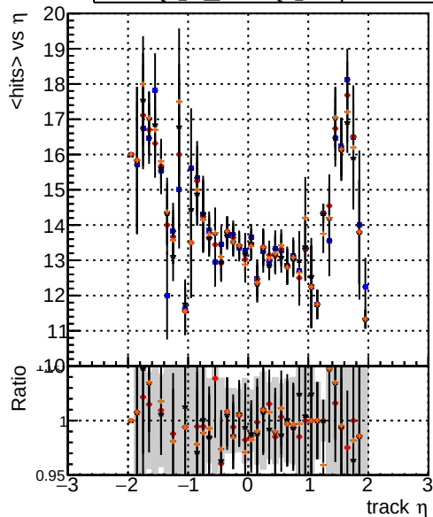
Legend: - DQM_TT_mkFit-DQM_original (blue line) - /data2/legianni/standalone-May24/CMSSW_13_2_X_2023-06-05-1100/src/DQM_TT_mkFit-DQM_mod_updatedmod127 (red line) - DQM_TT_mkFit-DQM_update-mod127 (black line) - DQM_TT_mkFit-DQM_127-updatemod127 (orange line)
