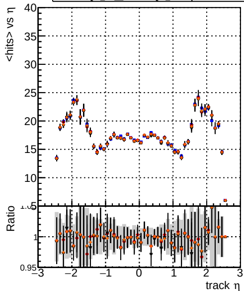
mean hits vs \eta Legend: - DQM_TT_mkFit-DQM_original (blue line with circles) - /data2/legianni/standalone-May24/CMSSW_13_2_X_2023-06-05-1100/src/DQM_TT_mkFit-DQM_mod_updatedmod127 (red line with circles) - DQM_TT_mkFit-DQM_update-mod127 (black line with circles) - DQM_TT_mkFit-DQM_127-updatemod127 (orange line with circles)
