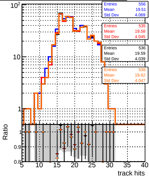
mean hit DQM TT mkFit-DQM original /data2/legianni/standalone-May24/CMSSW_13_2_X_2023-06-05-1100/src/DQM TT_mkFit-DQM_mod_updatedmod127 DQM TT_mkFit-DQM_update-mod127 DQM TT_mkFit-DQM_127-updatemod127
