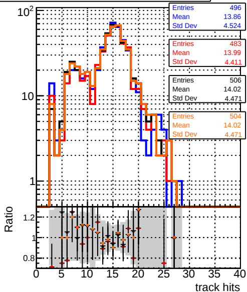
mean hits — DQM_TT_mkFit-DQM_original — /data2/legianni/standalone-May24/CMSSW_13_2_X_2023-06-05-1100/src/DQM_TT_mkFit-DQM_mod_updatedmod127 — DQM_TT_mkFit-DQM_update-mod127 — DQM_TT_mkFit-DQM_127-updatemod127
