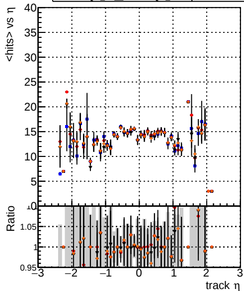
mean hits — DQM_TT_mkFit-DQM_original — /data2/legianni/standalone-May24/CMSSW_13_2_X_2023-06-05-1100/src/DQM_TT_mkFit-DQM_mod_updatedmod127 — DQM_TT_mkFit-DQM_update-mod127 — DQM_TT_mkFit-DQM_127-updatemod127
