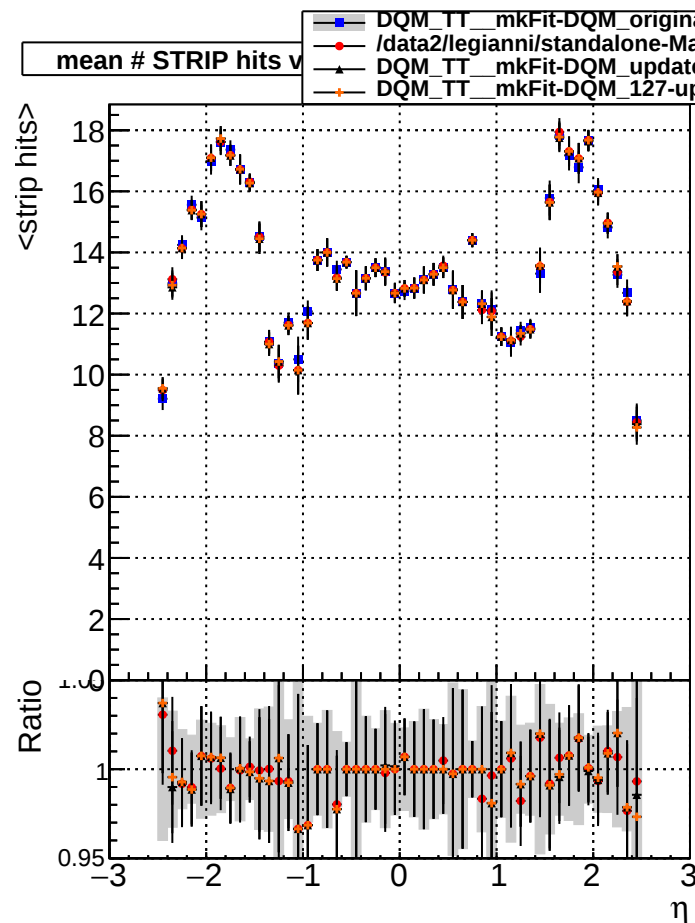
Legend: \blacksquare DQM_TT_mkFit-DQM_original \bullet /data2/legianni/standalone-May24/CMSSW_13_2_X_2023-06-05-1100/src/DQM_TT_mkFit-DQM_mod_upd \blacktriangle DQM_TT_mkFit-DQM_update-mod127 \blacklozenge DQM_TT_mkFit-DQM_127-updatemod127
