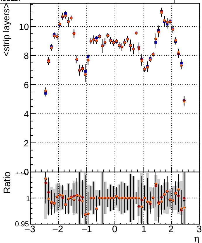
Legend: \blacksquare DQM_TT_mkFit-DQM_original \bullet /data2/legianni/standalone-May24/CMSSW_13_2_X_2023-06-05-1100/src/DQM_TT_mkFit-DQM_mod_upd \blacktriangle DQM_TT_mkFit-DQM_update-mod127 \blacklozenge DQM_TT_mkFit-DQM_127-updatemod127
