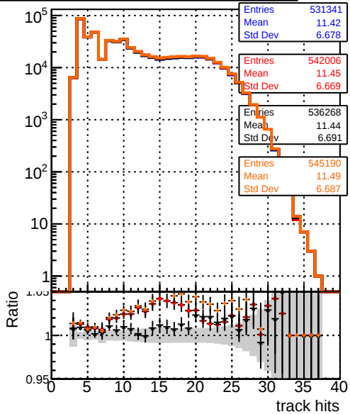
— DQM_TT_mkFit-DQM_original — /data2/legianni/standalone-May24/CMSSW_13_2_X_X-2023-06-05-1100/src/DQM_TT_mkFit-DQM_mod_updatedmod127 — DQM_TT_mkFit-DQM_update-mod127 — DQM_TT_mkFit-DQM_127-updatemod127
