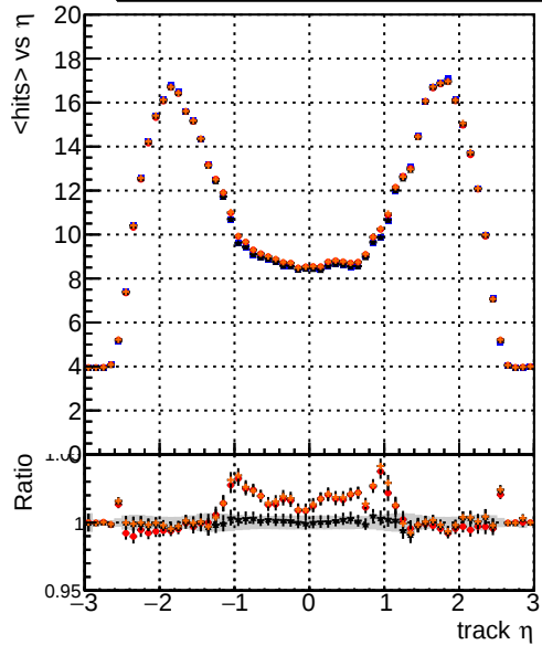
— DQM_TT_mkFit-DQM_original — /data2/legianni/standalone-May24/CMSSW_13_2_X_X-2023-06-05-1100/src/DQM_TT_mkFit-DQM_mod_updatedmod127 — DQM_TT_mkFit-DQM_update-mod127 — DQM_TT_mkFit-DQM_127-updatemod127
