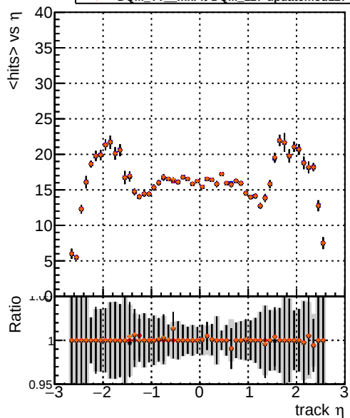
mean hits vs \eta Legend: DQM_TT_mkFit-DQM_original (blue line), /data2/legianni/standalone-May24/CMSSW_13_2_X_2023-06-05-1100/src/DQM_TT_mkFit-DQM_mod_updatedmod127 (red line), DQM_TT_mkFit-DQM_update-mod127 (black line), DQM_TT_mkFit-DQM_127-updatemod127 (orange line)
