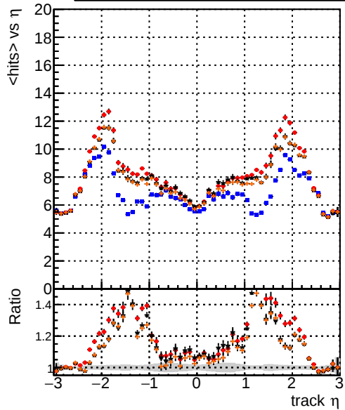
mean hits vs \eta — DQM TT mkFit-DQM original — /data2/legianni/standalone-May24/CMSSW_13_2_X_2023-06-05-1100/src/DQM TT_mkFit-DQM_mod_updatedmod-127 — DQM TT mkFit-DQM_update-mod127 — DQM TT mkFit-DQM_127-updatemod127
