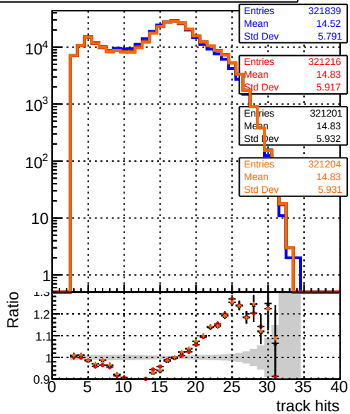
Legend: DQM TT mkFit-DQM original (blue), /data2/legianni/standalone-May24/CMSSW_13_2_X_2023-06-05-1100/src/DQM TT mkFit-DQM_mod_updatedmod-127 (red), DQM TT mkFit-DQM_update-mod127 (black), DQM TT mkFit-DQM_127-updatemod127 (orange)
