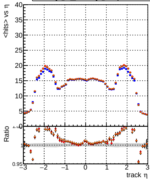
Legend: DQM TT mkFit-DQM original (blue), /data2/legianni/standalone-May24/CMSSW_13_2_X_2023-06-05-1100/src/DQM TT mkFit-DQM_mod_updatedmod-127 (red), DQM TT mkFit-DQM_update-mod127 (black), DQM TT mkFit-DQM_127-updatemod127 (orange)
