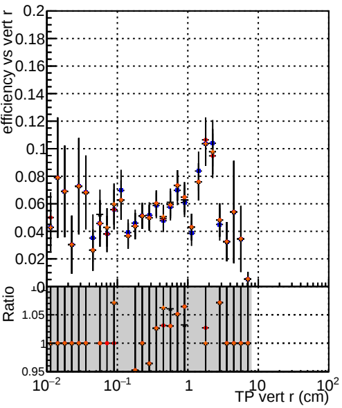
Efficiency vs TP vert r (cm) - Legend — DQM TT mkFit-DQM original — /data2/legianni/standalone-May24/CMSSW_13_2_X_2023-06-05-1100/src/DQM TT_mkFit-DQM_mod_updatedmod-127 — DQM TT_mkFit-DQM_update-mod127 — DQM TT_mkFit-DQM_127-updatemod127
