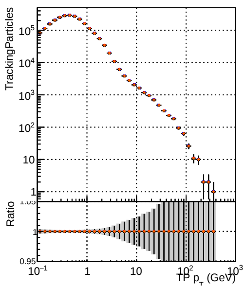
Legend: - blue circle: DQM_TT_mkFit-DQM_original - red diamond: /data2/legianni/standalone-May24/CMSSW_13_2_X_2023-06-05-1100/src/DQM_TT_mkFit-DQM_mod_updatedmod127 - black triangle: DQM_TT_mkFit-DQM_update-mod127 - orange star: DQM_TT_mkFit-DQM_127-updatemod127
