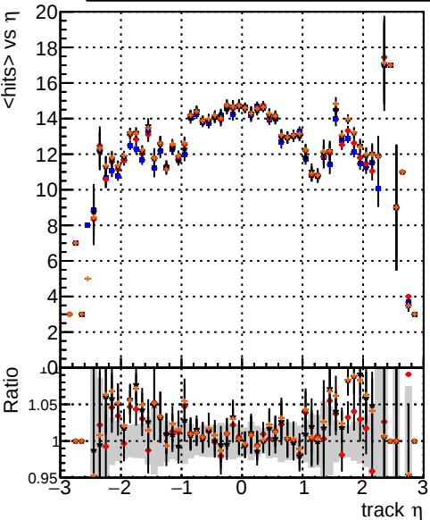
mean hit — DQM_TT_mkFit-DQM_original — /data2/legianni/standalone-May24/CMSSW_13_2_X_2023-06-05-1100/src/DQM_TT_mkFit-DQM_mod_updatedmod-127 — DQM_TT_mkFit-DQM_update-mod127 — DQM_TT_mkFit-DQM_127-updatemod127
