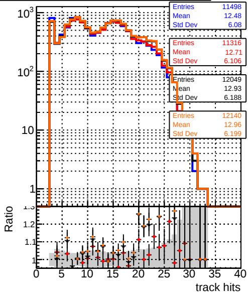
mean hit — DQM_TT_mkFit-DQM_original — /data2/legianni/standalone-May24/CMSSW_13_2_X_2023-06-05-1100/src/DQM_TT_mkFit-DQM_mod_updatedmod-127 — DQM_TT_mkFit-DQM_update-mod127 — DQM_TT_mkFit-DQM_127-updatemod127
