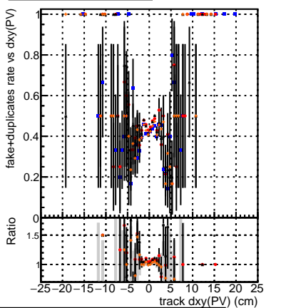
fake+duplicates vs dxy(PV)
