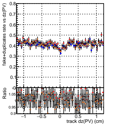
fake+duplicates vs dz(PV)
