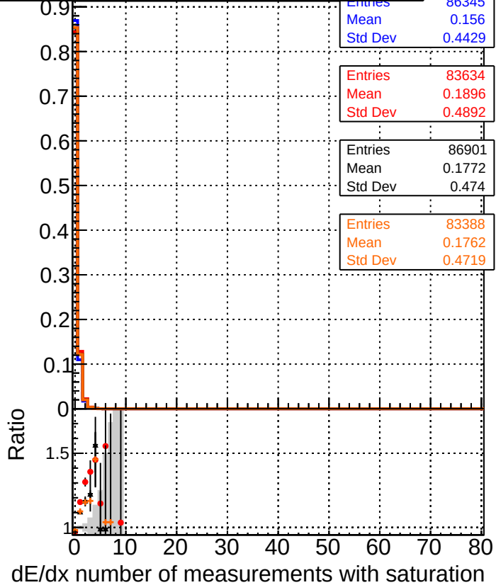
Legend: — DQM_TT mkFit-DQM_original (blue line) — /data2/legianni/standalone-May24/CMSSW_13_2_X_2023-06-05-1100/src/DQM_TT_mkFit-DQM_mod_upd (red line with dots) — DQM_TT mkFit-DQM_update-mod127 (black line with dots) — DQM_TT mkFit-DQM_127-updatemod127 (orange line with dots)
