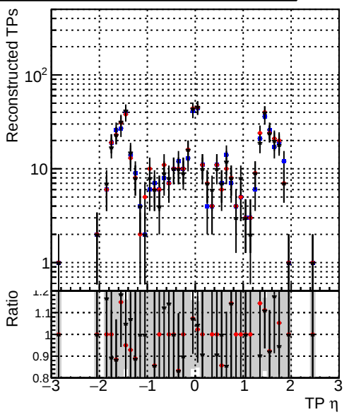
Legend: - blue dots: DQM_TT_mkFit-DQM_original - red dots: /data2/legianni/standalone-May24/CMSSW_13_2_X_2023-06-05-1100/src/DQM_TT_mkFit-DQM_mod_updatedmod-127 - black dots: DQM_TT_mkFit-DQM_update-mod127
