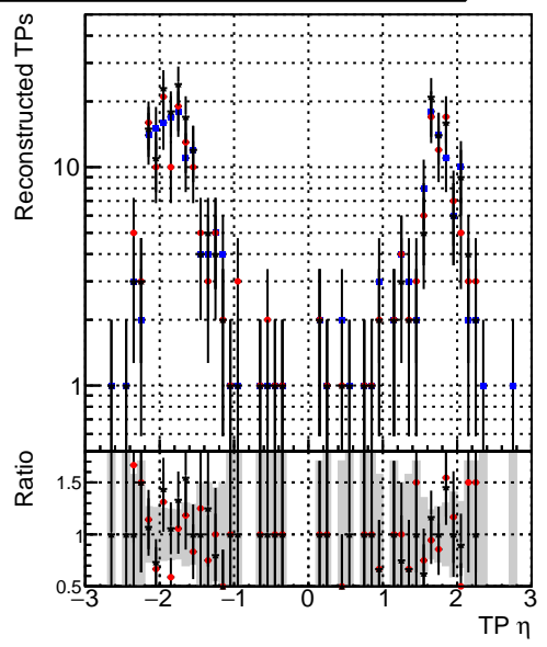
N of simulated tracks vs \eta Legend: \bullet DQM_TT_mkFit-DQM_original \bullet /data2/legianni/standalone-May24/CMSSW_13_2_X_2023-06-05-1100/src/DQM_TT_mkFit-DQM_mod_updatedmod-127 \bullet DQM_TT_mkFit-DQM_update-mod127
