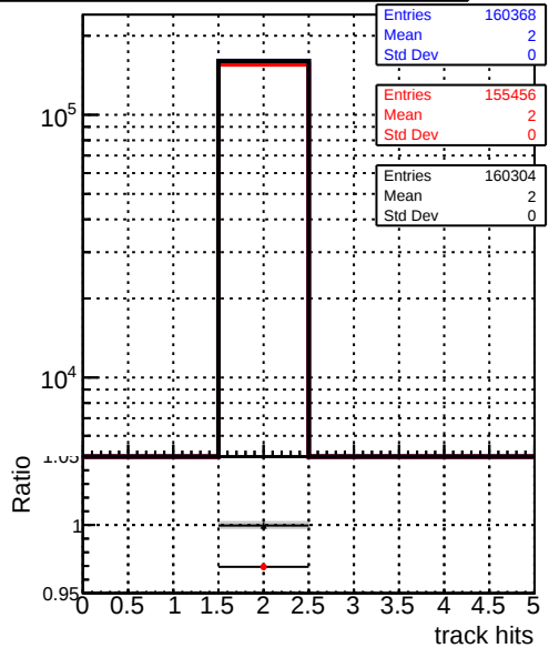
mean hits Legend: DQM_TT_mkFit-DQM_original (blue line), /data2/legianni/standalone-May24/CMSSW_13_2_X_2023-06-05-1100/src/DQM_TT_mkFit-DQM_mod_updatedmod-127 (red line), DQM_TT_mkFit-DQM_update-mod127 (black line)
