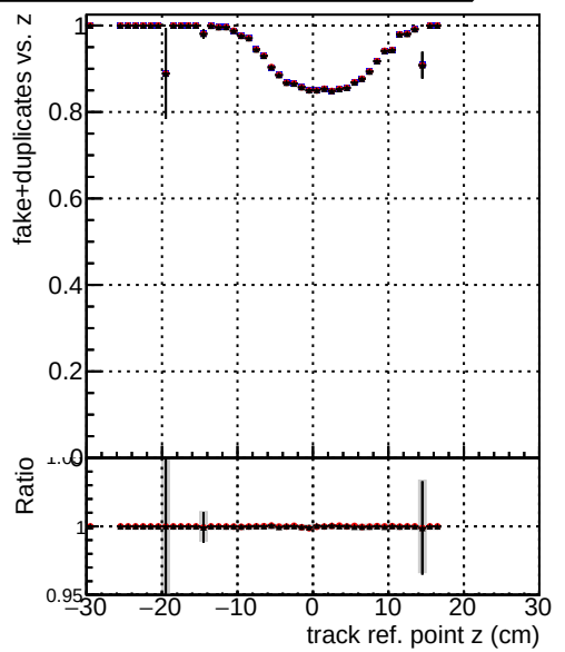
Legend: DQM_TT_mkFit-DQM_original /data2/legianni/standalone-May24/CMSSW_13_2_X_2023-06-05-1100/src/DQM_TT_mkFit-DQM_mod_updatedmod-127 DQM_TT_mkFit-DQM_update-mod127
