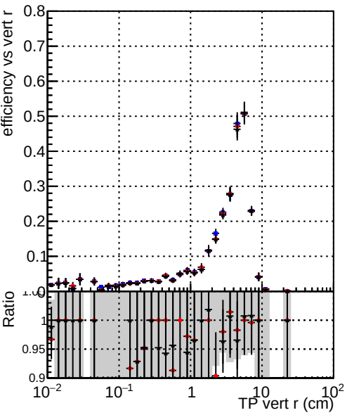
Legend: - blue circles: DQM_TT_mkFit-DQM_original - red circles: /data2/legianni/standalone-May24/CMSSW_13_2_X_2023-06-05-1100/src/DQM_TT_mkFit-DQM_mod_updatedmod-127 - black circles: DQM_TT_mkFit-DQM_update-mod127
