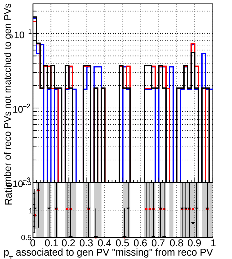
RecoPVAssoc2GenPVNotMatched_missing
