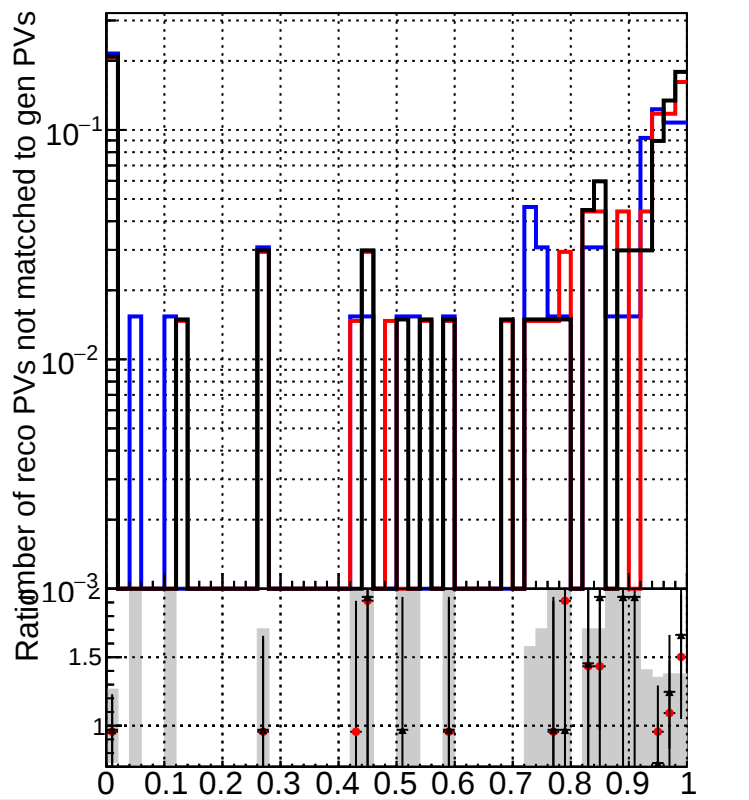
RecoPVAssoc2GenPVNotMatched_Purity
