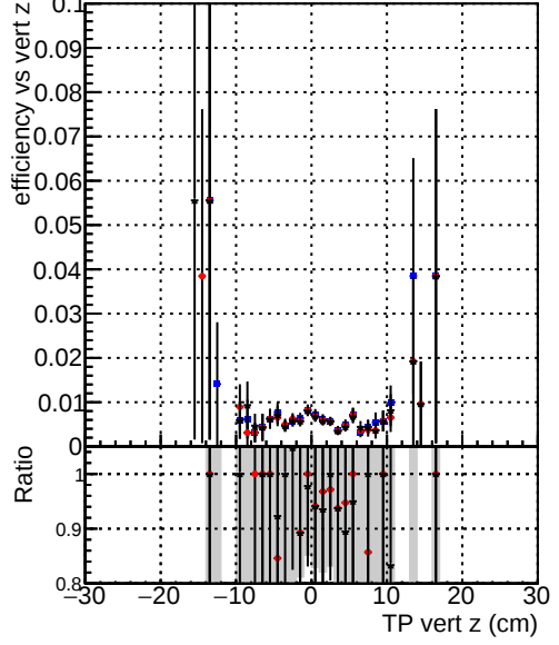
Efficiency vs. TP vert z (cm) for DQM_TT_mkFit-DQM_update-mod127
