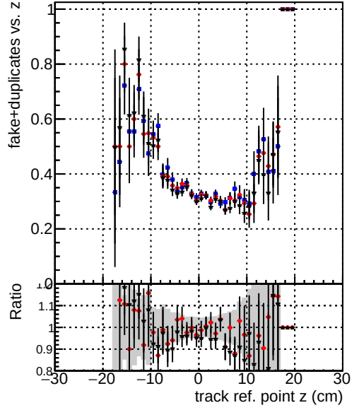
—●— DQM_TT_mkFit-DQM_original —●— /data2/legianni/standalone-May24/CMSSW_13_2_X_2023-06-05-1100/src/DQM_TT_mkFit-DQM_mod_updatedmod-127 —●— DQM_TT_mkFit-DQM_update-mod127
