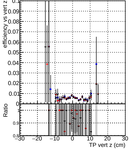
—●— DQM_TT_mkFit-DQM_original —●— /data2/legianni/standalone-May24/CMSSW_13_2_X_2023-06-05-1100/src/DQM_TT_mkFit-DQM_mod_updatedmod-127 —●— DQM_TT_mkFit-DQM_update-mod127
