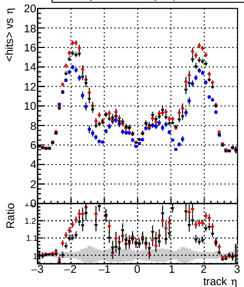
mean hits vs \eta — DQM_TT_mkFit-DQM_original — /data2/legianni/standalone-May24/CMSSW_13_2_X_2023-06-05-1100/src/DQM_TT_mkFit-DQM_mod_updatedmod-127 — DQM_TT_mkFit-DQM_update-mod127
