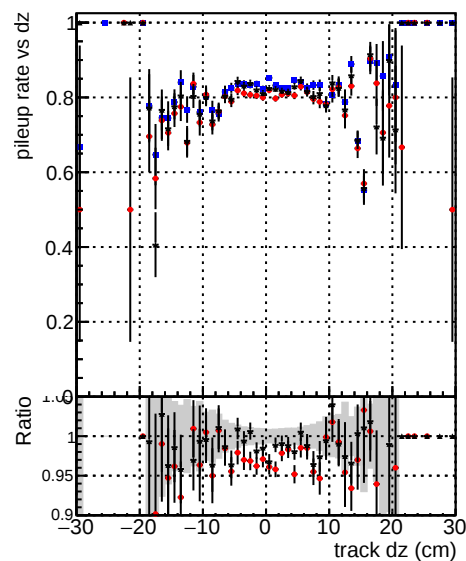
24/CMSSW_13_2_X_2023-06-05-1100/src/DQM_TT__mkFit-DQM_mod_updatedmod-127 mod127
