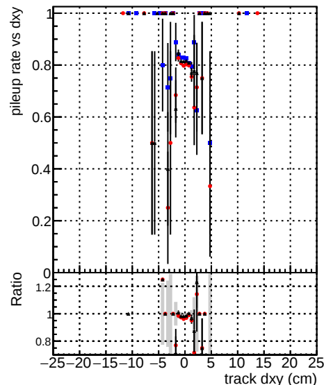
24/CMSSW_13_2_X_2023-06-05-1100/src/DQM_TT__mkFit-DQM_mod_updatedmod-127 mod127
