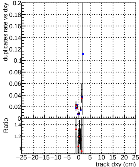
24/CMSSW_13_2_X_2023-06-05-1100/src/DQM_TT__mkFit-DQM_mod_updatedmod-127 mod127
