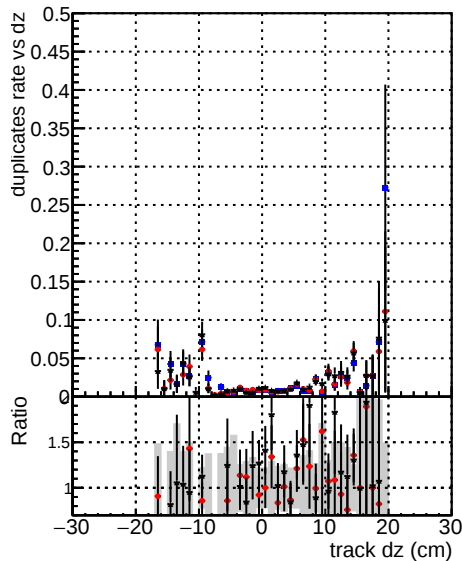
24/CMSSW_13_2_X_2023-06-05-1100/src/DQM_TT__mkFit-DQM_mod_updatedmod-127 mod127
