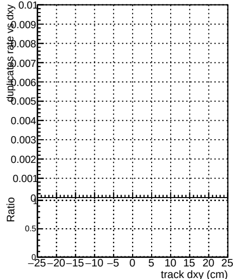
4/CMSSW_13_2_X_2023. mod127
