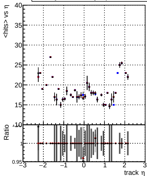
mean hits — DQM_TT_mkFit-DQM_original — /data2/legianni/standalone-May24/CMSSW_13_2_X_2023-06-05-1100/src/DQM_TT_mkFit-DQM_mod_updatedmod127 — DQM_TT_mkFit-DQM_update-mod127
