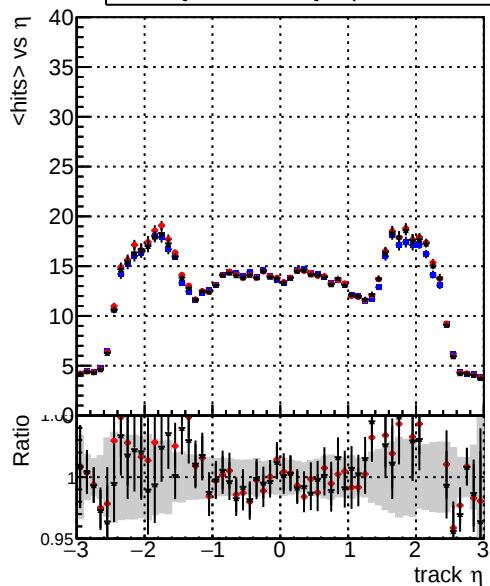
mean hits vs \eta — DQM_TT_mkFit-DQM_original — /data2/legianni/standalone-May24/CMSSW_13_2_X_2023-06-05-1100/src/DQM_TT_mkFit-DQM_mod_updatedmod127 — DQM_TT_mkFit-DQM_update-mod127
