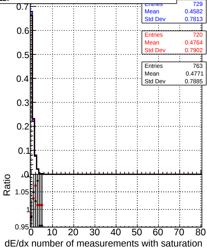
/data2/legianni/standalone-May24/CMSSW_13_2_X_2023-06-05-1100/src/DQM_TT_mkFit-DQM_mod_upd
