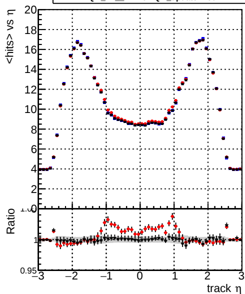
mean hits vs \eta Legend: DQM_TT_mkFit-DQM_original (blue line), /data2/legianni/standalone-May24/CMSSW_13_2_X_2023-06-05-1100/src/DQM_TT_mkFit-DQM_mod_updatedmod-127 (red line), DQM_TT_mkFit-DQM_update-mod127 (black line)
