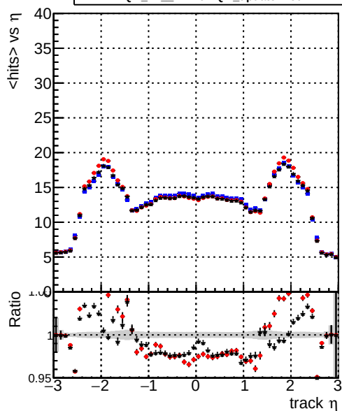
mean hits vs \eta — DQM_TT_mkFit-DQM_original — /data2/legianni/standalone-May24/CMSSW_13_2_X_2023-06-05-1100/src/DQM_TT_mkFit-DQM_mod_updatedmod127 — DQM_TT_mkFit-DQM_update-mod127
