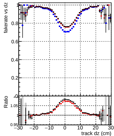
Fake rate vs dz Legend: DOM TT mkFit-DQM original data2/legiannijustalone-May24/CMSSW_13_2_X_2023-06-05-1100/src/DQM TT_mkFit-DQM_mod_updatedmod-127 DOM TT mkFit-DQM update-mod127
