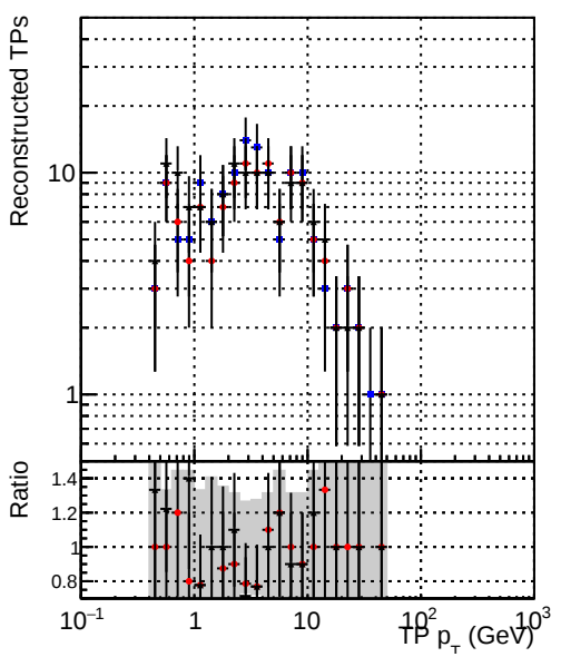
Legend: - \bullet DQM_TT_mkFit-DQM_original - \bullet /data2/legianni/standalone-May24/CMSSW_13_2_X_2023-06-05-1100/src/DQM_TT_mkFit-DQM_mod_updatedmod-127 - \bullet DQM_TT_mkFit-DQM_update-mod127
