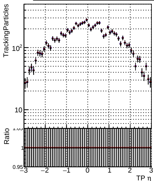
Legend: - \bullet DQM_TT_mkFit-DQM_original - \bullet /data2/legianni/standalone-May24/CMSSW_13_2_X_2023-06-05-1100/src/DQM_TT_mkFit-DQM_mod_updatedmod-127 - \bullet DQM_TT_mkFit-DQM_update-mod127
