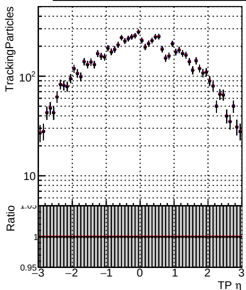
—•— DQM_TT_mkFit-DQM_original —•— /data2/legianni/standalone-May24/CMSSW_13_2_X_2023-06-05-1100/src/DQM_TT_mkFit-DQM_mod_updatedmod-127 —•— DQM_TT_mkFit-DQM_update-mod127
