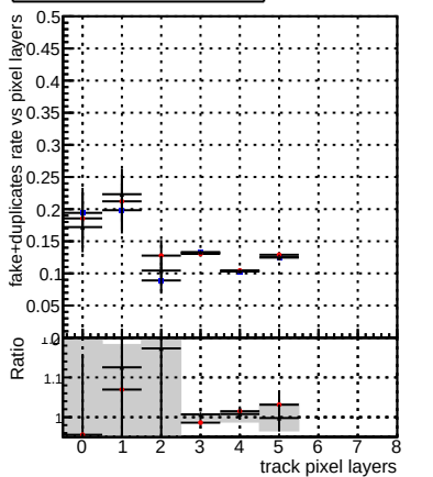
fake+duplicates vs pixel layers
