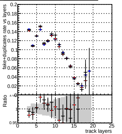
fake+duplicates vs layers
