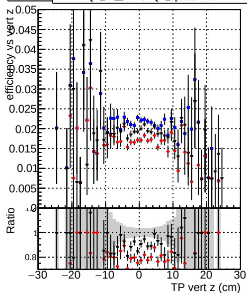
Efficiency vs TP vert z —●— DQM_TT_mkFit-DQM_original —★— /data2/legianni/standalone-May24/CMSSW_13_2_X_2023-06-05-1100/src/DQM_TT_mkFit-DQM_mod_updatedmod-127 —★— DQM_TT_mkFit-DQM_update-mod127
