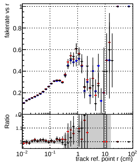
—●— DQM TT mkFit-DQM original —●— /data2/legianni/standalone-May24/CMSSW_13_2_X_2023-06-05-1100/src/DQM TT_mkFit-DQM_mod_updatedmod127 —●— DQM TT_mkFit-DQM_update-mod127
