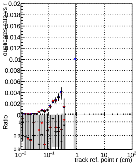
—●— DQM TT mkFit-DQM original —●— /data2/legianni/standalone-May24/CMSSW_13_2_X_2023-06-05-1100/src/DQM TT_mkFit-DQM_mod_updatedmod127 —●— DQM TT_mkFit-DQM_update-mod127
