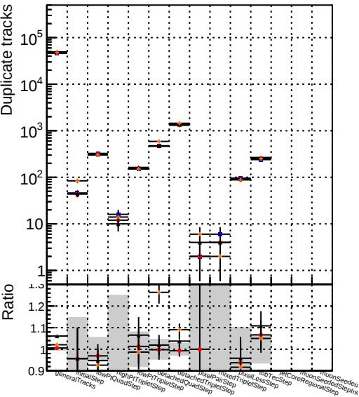
Legend: Blue circle: DQM TT mkFit-DQM_original Red circle: /data2/legianni/standalone-May24/CMSSW_13_2_X_2023-06-05-1100/src/DQM TT mkFit-DQM_updated0 Green circle: DQM TT mkFit-DQM_original_newwindows Orange circle: DQM TT mkFit-DQM_update-mod127
