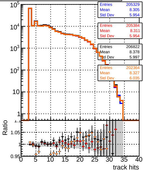
— DQM_TT_mkFit-DQM_original — /data2/legianni/standalone-May24/CMSSW_13_2_X_2023-06-05-1100/src/DQM_TT_mkFit-DQM_updated-0 — DQM_TT_mkFit-DQM_original_newwndows — DQM_TT_mkFit-DQM_update-mod127
