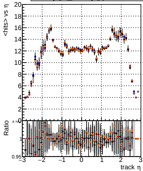
Legend for mean hits vs \eta : Blue line: DQM_TT_mkFit-DQM_original Red line with error bars: /data2/legianni/standalone-May24/CMSSW_13_2_X_2023-06-05-1100/src/DQM_TT_mkFit-DQM_updated-0 Black line with error bars: DQM_TT_mkFit-DQM_original_newwindows Orange line with error bars: DQM_TT_mkFit-DQM_update-mod127
