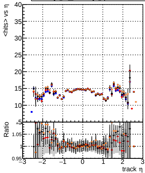
mean hits vs \eta Legend: DQM_TT_mkFit-DQM_original, /data2/legianni/standalone-May24/CMSSW_13_2_X_2023-06-05-1100/src/DQM_TT_mkFit-DQM_updated-0, DQM_TT_mkFit-DQM_original_newwindows, DQM_TT_mkFit-DQM_update-mod127
