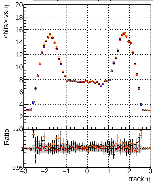
mean hits vs \eta Legend: DQM_TT_mkFit-DQM_original (blue line), /data2/legianni/standalone-May24/CMSSW_13_2_X_2023-06-05-1100/src/DQM_TT_mkFit-DQM_updated-0 (red line with dots), DQM_TT_mkFit-DQM_original_newwindows (black line with dots), DQM_TT_mkFit-DQM_update-mod127 (orange line with dots)
