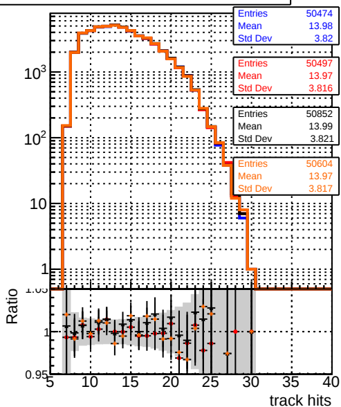
— DQM_TT_mkFit-DQM_original — /data2/legianni/standalone-May24/CMSSW_13_2_X_X-2023-06-05-1100/src/DQM_TT_mkFit-DQM_updated-0 — DQM_TT_mkFit-DQM_original_newwindows — DQM_TT_mkFit-DQM_update-mod127
